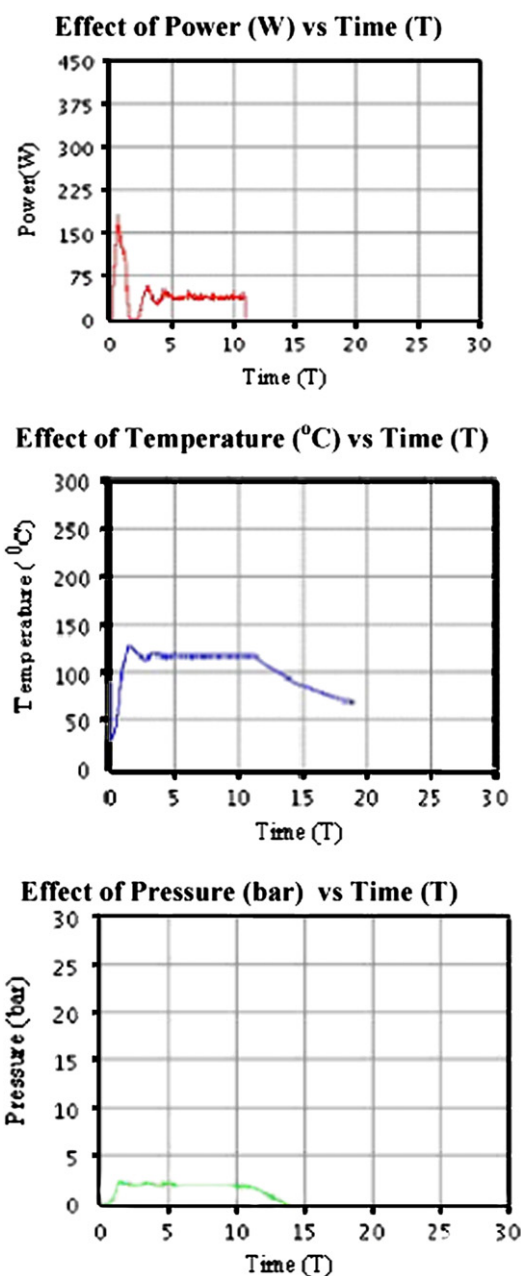
Fig. 1. Graphs A, B and C which summarize variation of power, temperature and pressure against time respectively during the reaction.
