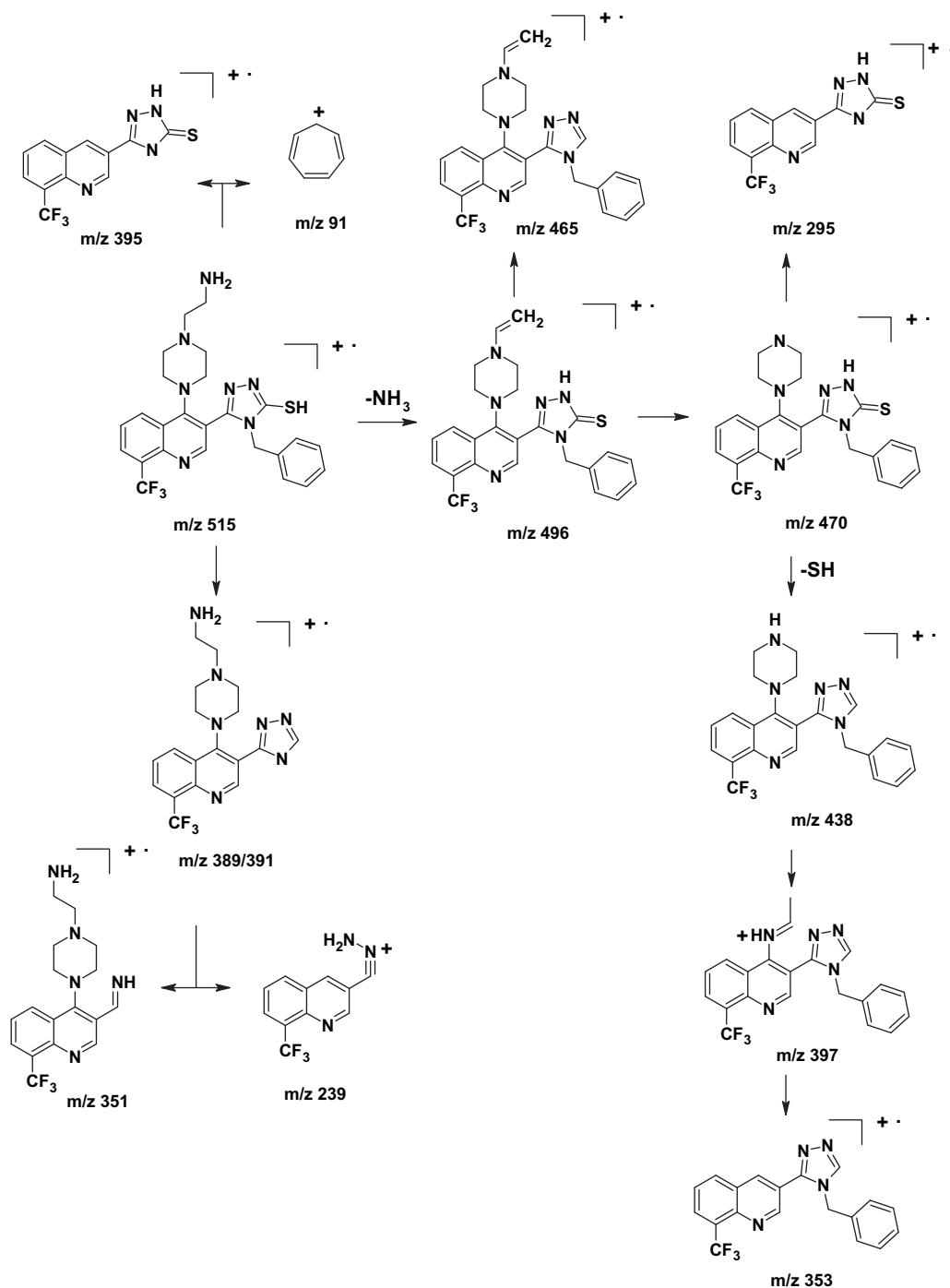
Scheme 2. Mass fragmentation pattern of compound 8g.
